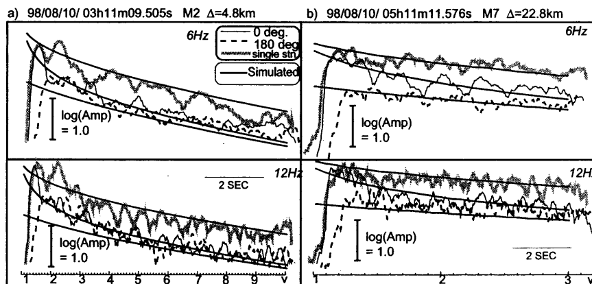
Figure 5. Envelopes observed and theoretically expected for 6 and 12 Hz ranges. a) and b) are those for epicentral distance of 4.8 and 22.8 km, respectively. Gray lines are envelopes of the single station record. Solid and dashed lines are slant-stacked envelopes in the direction of 0 and 180^\circ . Thick solid lines are theoretical curves of the single isotropic scattering model.
