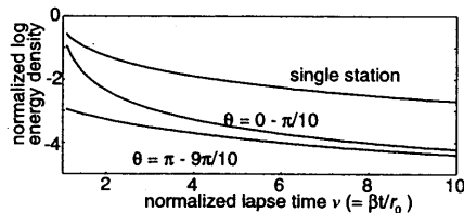
Figure 2. Envelopes calculated from formula (4). The curves show the cases of single station record and slant-stacked ones. The slant-stacking directions face to hypocenter and back to that, respectively.
